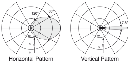
880 – 960 MHz: +45°/–45° Polarization
