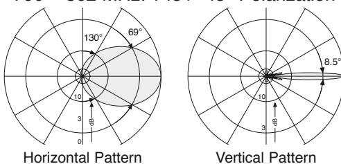
790 – 862 MHz: +45°/–45° Polarization
