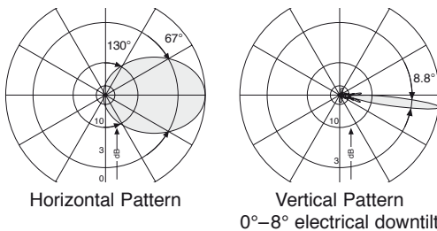
790 – 862 MHz: +45°/–45° Polarization
