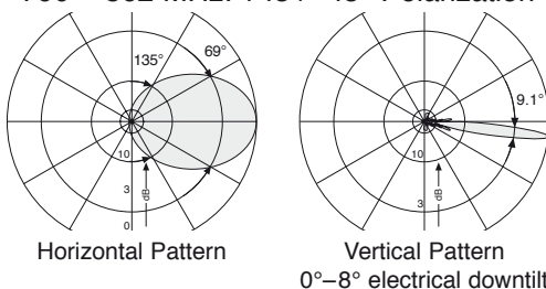
790 – 862 MHz: +45°/–45° Polarization
