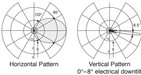
824 – 894 MHz: +45°/–45° Polarization
